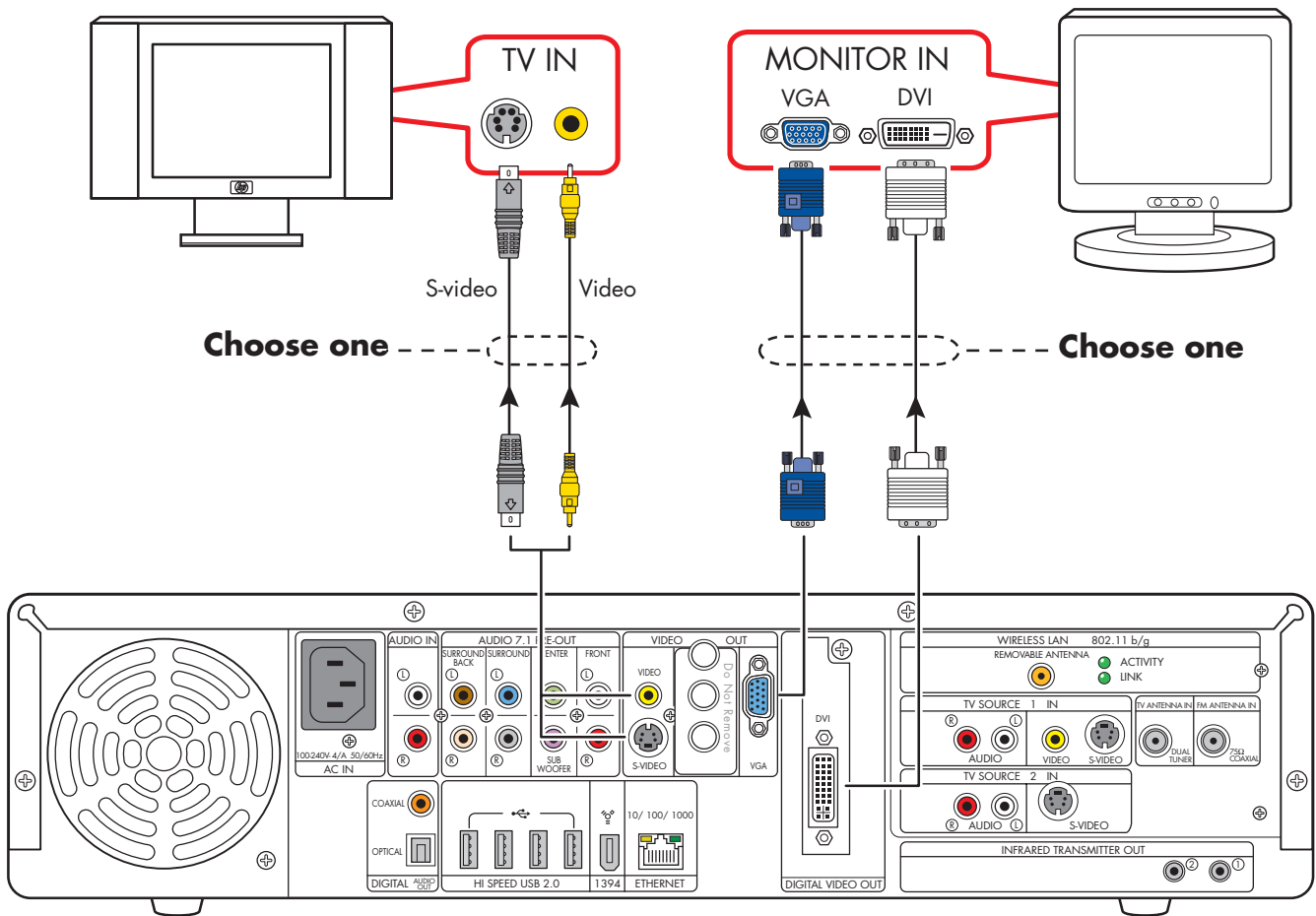
TV (standard definition shown) and monitor out
